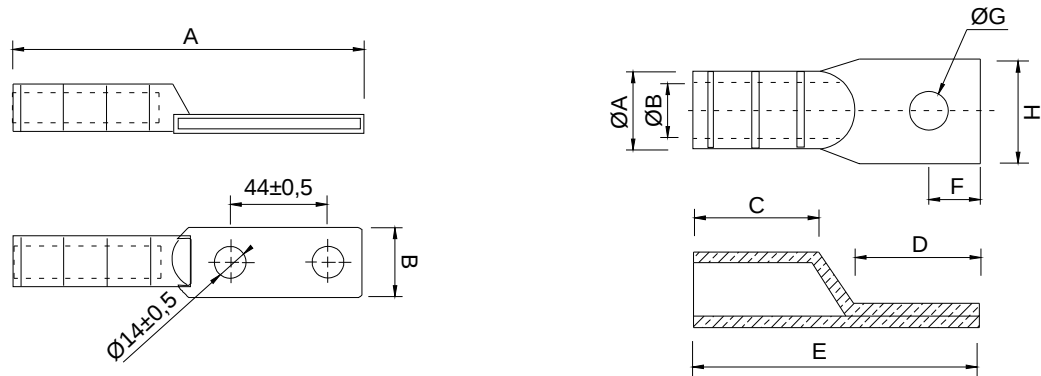
Figura 50 - Conector terminal
